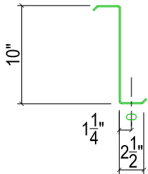
FLANGE PUNCHING 9/16" x 1" SLOTS (OPTIONAL)
