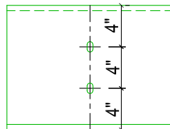
WEB PUNCHING 5/8" x 3/4" SLOTS (STANDARD)
