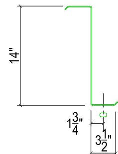
FLANGE PUNCHING 9/16" x 1" SLOTS (OPTIONAL)
