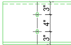
WEB PUNCHING 5/8" x 3/4" SLOTS (STANDARD)
