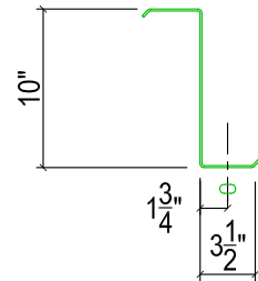
FLANGE PUNCHING 9/16" x 1" SLOTS (OPTIONAL)
