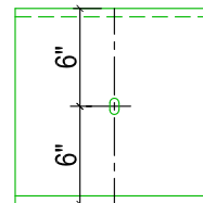
SAG ROD PUNCHING 5/8" x 3/4" SLOTS (OPTIONAL)
