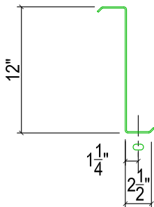
FLANGE PUNCHING 9/16" x 1" SLOTS (OPTIONAL)
