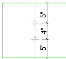
WEB PUNCHING 5/8" x 3/4" SLOTS (STANDARD)
