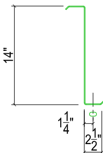
FLANGE PUNCHING 9/16" x 1" SLOTS (OPTIONAL)
