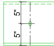
SAG ROD PUNCHING 5/8" x 3/4" SLOTS (OPTIONAL)
