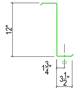
FLANGE PUNCHING 9/16" x 1" SLOTS (OPTIONAL)
