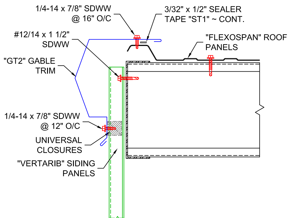
GABLE DETAIL
