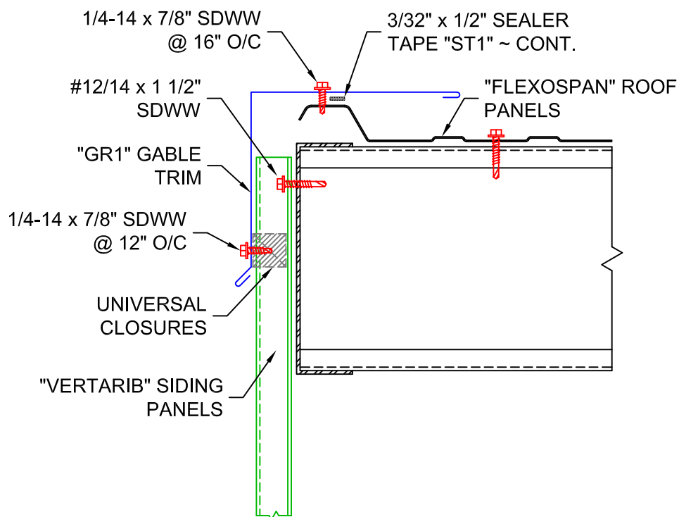
GABLE DETAIL
