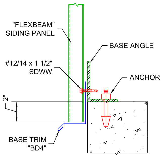
CURB w/ TRIM
