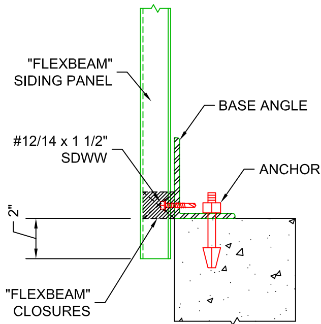
CURB w/ CLOSURE
