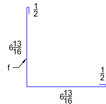
"OS2" OUTSIDE CORNER TRIM
