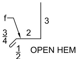
"BD6" BASE TRIM
