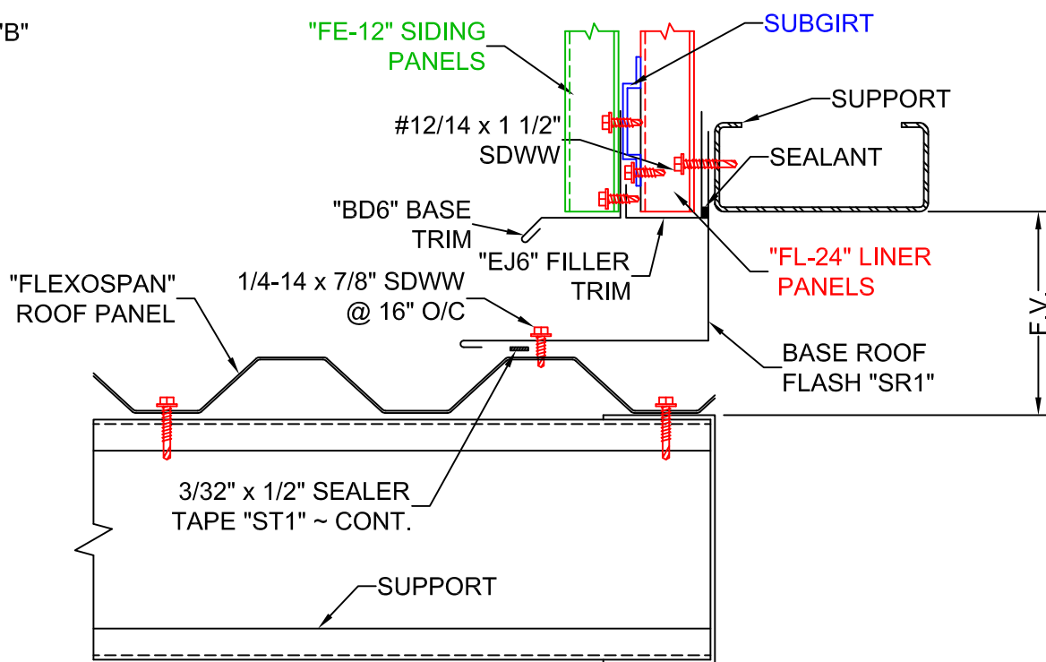
"EJ6" FILLER TRIM
