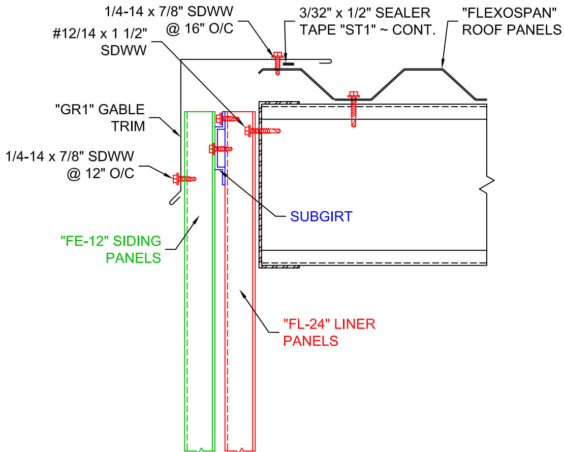
GABLE DETAIL
