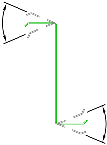
ZEE EAVE STRUTS (BOTH FLANGES OR ONE CAN BE PITCHED)
