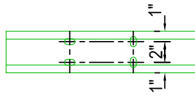
WEB PUNCHING 5/8" x 3/4" SLOTS (STANDARD)
