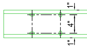
WEB PUNCHING 5/8" x 3/4" SLOTS (STANDARD)
