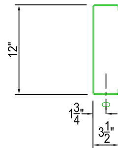
FLANGE PUNCHING 9/16" x 1" SLOTS (OPTIONAL)
