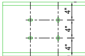
WEB PUNCHING 5/8" x 3/4" SLOTS (STANDARD)
