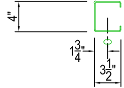
FLANGE PUNCHING 9/16" x 1" SLOTS (OPTIONAL)
