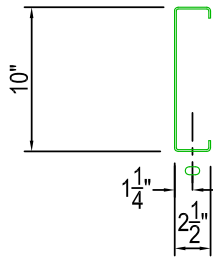
FLANGE PUNCHING 9/16" x 1" SLOTS (OPTIONAL)
