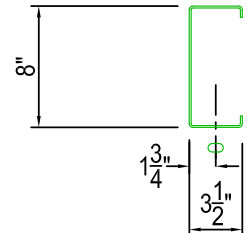
FLANGE PUNCHING 9/16" x 1" SLOTS (OPTIONAL)
