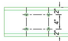
WEB PUNCHING 5/8" x 3/4" SLOTS (STANDARD)
