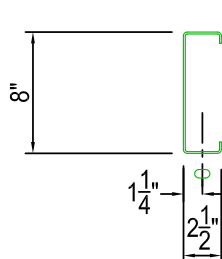
FLANGE PUNCHING 9/16" x 1" SLOTS (OPTIONAL)
