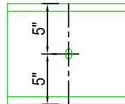
SAG ROD PUNCHING 5/8" x 3/4" SLOTS (OPTIONAL)
