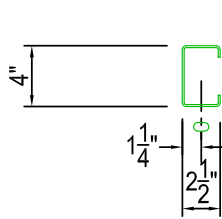
FLANGE PUNCHING 9/16" x 1" SLOTS (OPTIONAL)
