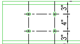
WEB PUNCHING 5/8" x 3/4" SLOTS (STANDARD)
