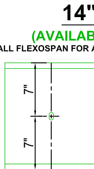
SAG ROD PUNCHING 5/8" x 3/4" SLOTS (OPTIONAL)
