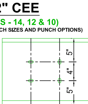
WEB PUNCHING 5/8" x 3/4" SLOTS (STANDARD)
