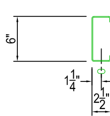
FLANGE PUNCHING 9/16" x 1" SLOTS (OPTIONAL)
