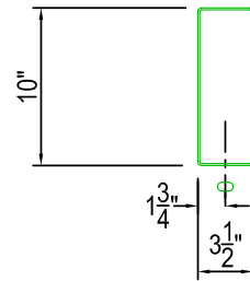
FLANGE PUNCHING 9/16" x 1" SLOTS (OPTIONAL)
