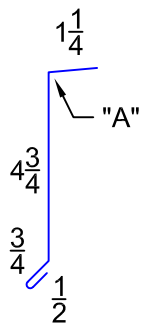
"LE3" EAVE TRIM
