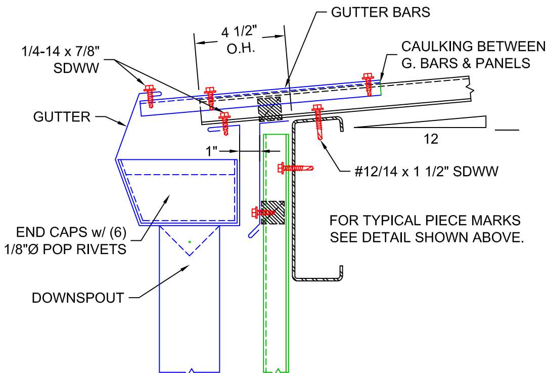
EAVE w/ TRIM & GUTTER
