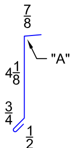
"LE2" EAVE TRIM
