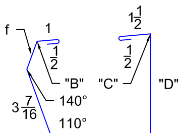
"SSGU2" GUTTER
