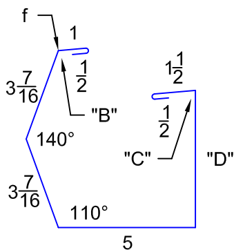
"GU1" GUTTER
