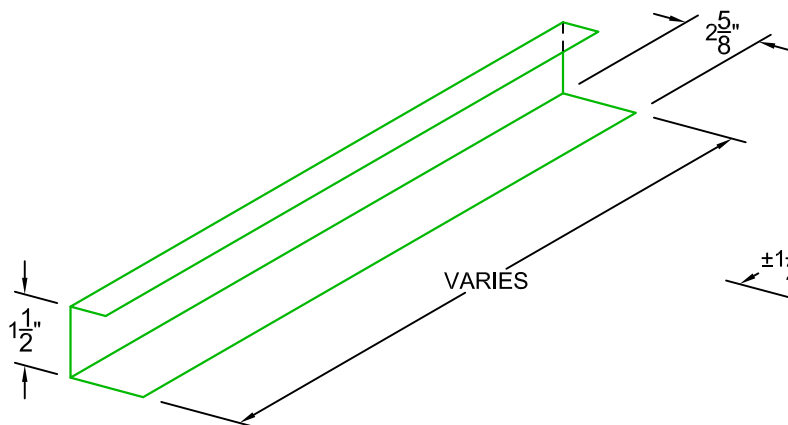
STEP 1: FIELD CUT (PANEL WIDTH + 3") PIECES FROM 10'-0" SECTIONS.
