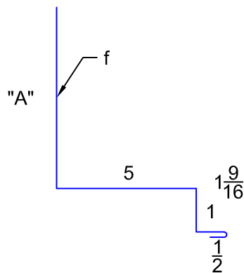
"FSS15-12" BASE ROOF TRIM
