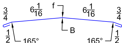
"RC1" RIDGE CAP
