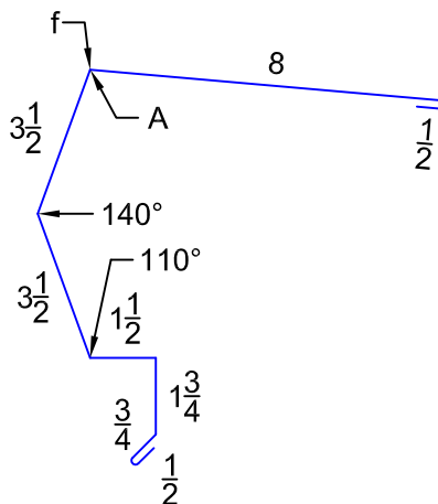
"GT3" HI-EAVE TRIM
