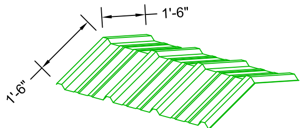
"RC2" FORMED RIDGE CAP
