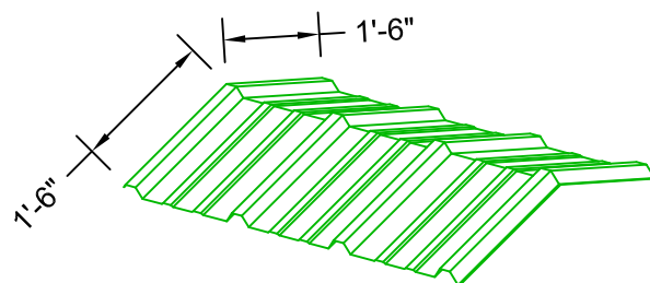
"FRRRC2" FORMED RIDGE CAP
