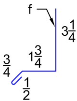
"BD5" BASE TRIM
