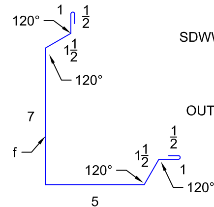
"OS3" OUTSIDE CORNER TRIM
