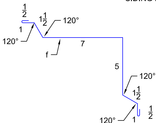
"IS3" INSIDE CORNER TRIM
