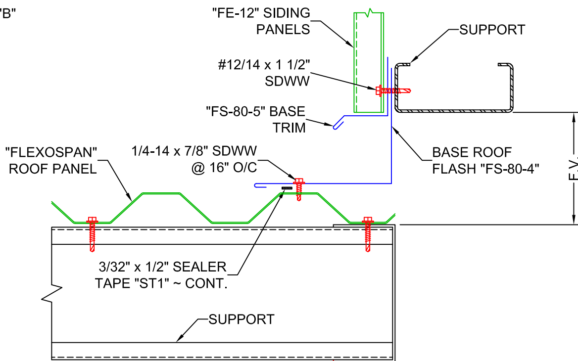
"FS-80-4" BASE ROOF FLASH
