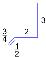
"FS-80-5" BASE TRIM
