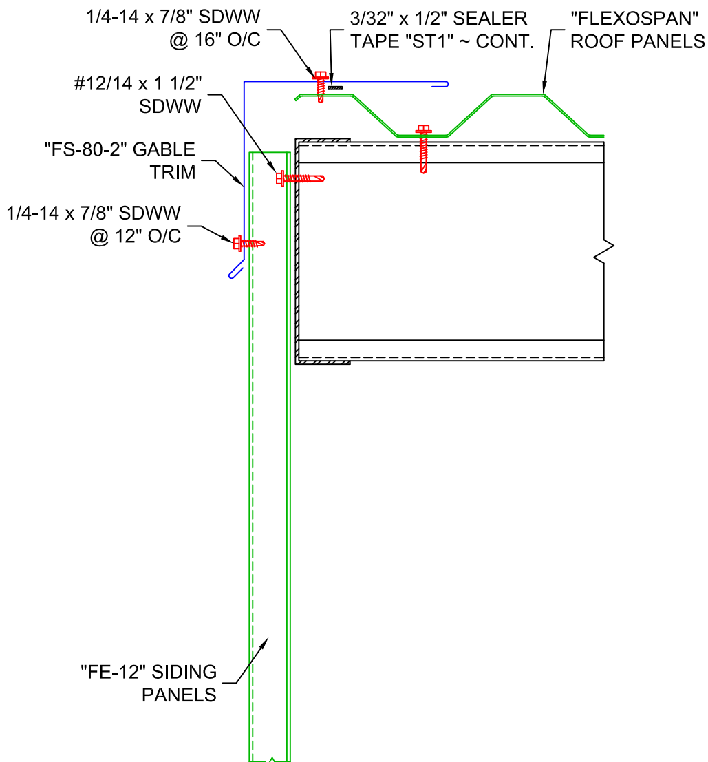
GABLE DETAIL
