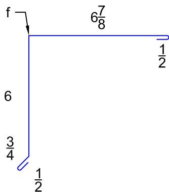
"FS-80-2" GABLE TRIM
