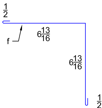
"IS2" INSIDE CORNER TRIM
