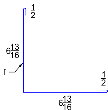
"OS2" OUTSIDE CORNER TRIM
